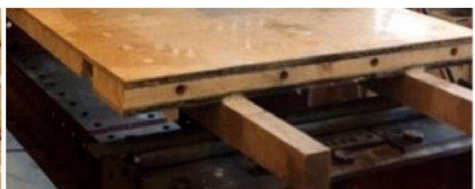
Figure 4. The two types of formwork elements: A-series (left) consists of formwork elements with full cross sections, B-series (right) consists of formwork elements on sample scale.
