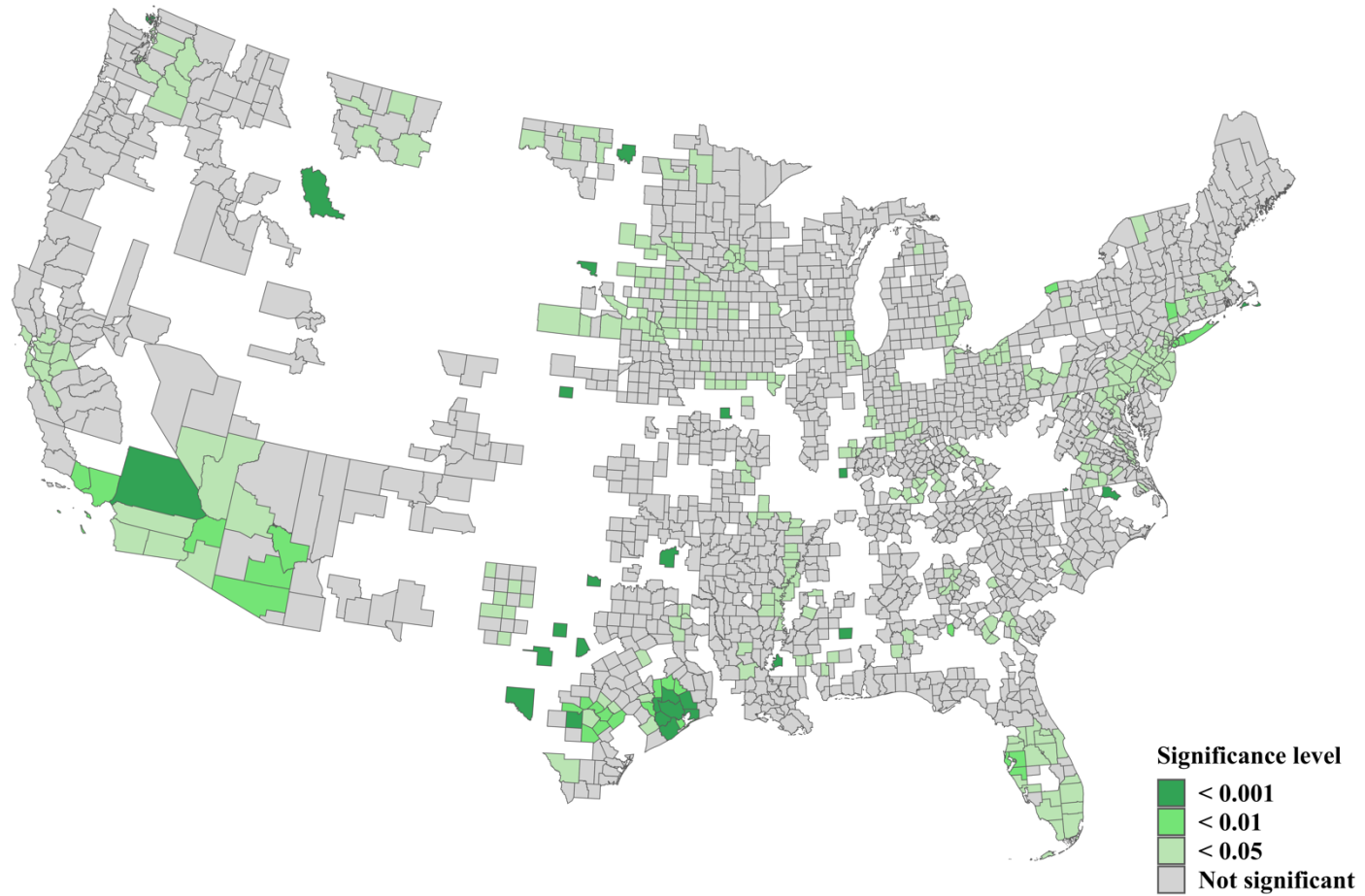
Figure A2. The LISA significance map of newspaper circulation changes in the U.S. (2018 - 2022)
