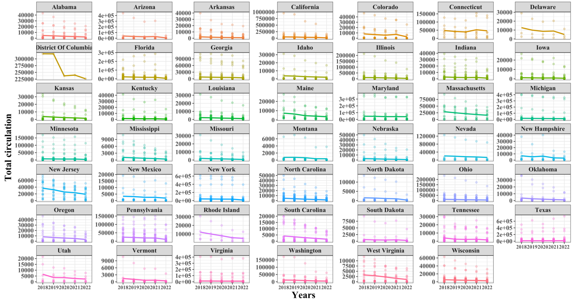
Figure A1. The newspaper circulation aggregated on the state level in the U.S. (2018 - 2022)
